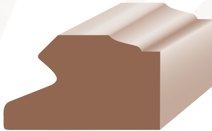
15/16 x 1-9/16 Stucco Mold
