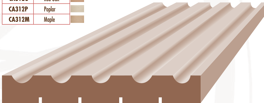
1/2 x 3-1/2 Fluting
