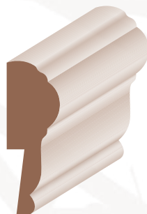
13/16 x 2-3/8 (5/16 Rabbet)
